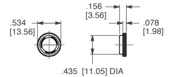
PANEL DRESS NUT
